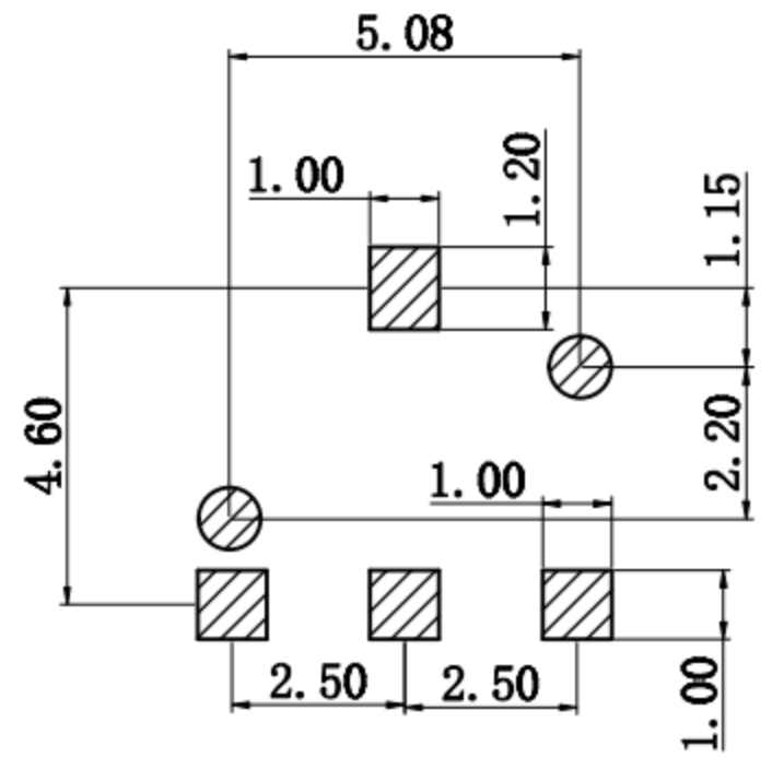
PCB Layout
